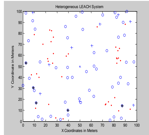
Figure 6: Simulation result after 1200 rounds in Proposed LEACH-Heterogeneous System. (Nearly 35 nodes are died)
