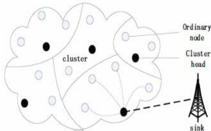
Figure 1. LEACH Protocol
