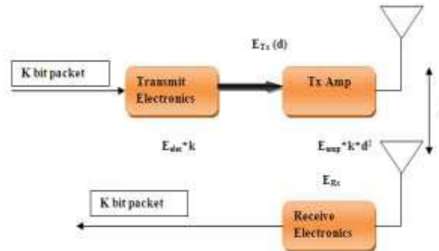
Figure 2. First Order Radio Energy Model
